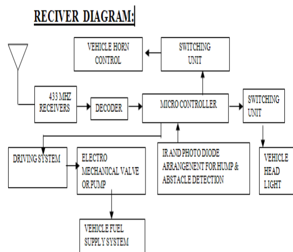
Fig1. Block diagram of Receiver
